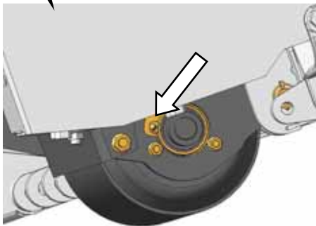
OPTIONAL GAUGE ROLL BEARINGS (2 PLCS) BOTH SIDES – 16 FT ONLY
